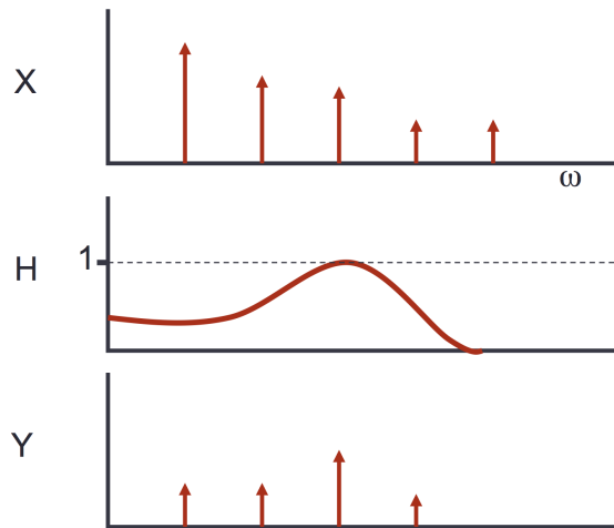
Figure 4: Filtering in the frequency domain. The input signal with spectrum X is multiplied by the frequency response of the filter H to obtain the output spectrum Y . The result of filtering is to reduce the amplitude of some frequencies and boost the amplitudes of others. In addition to amplitude changes, filters nearly always cause phase shifts that are also frequency dependent. Since we are much less sensitive to phase, we usually ignore the phase response of filters.
