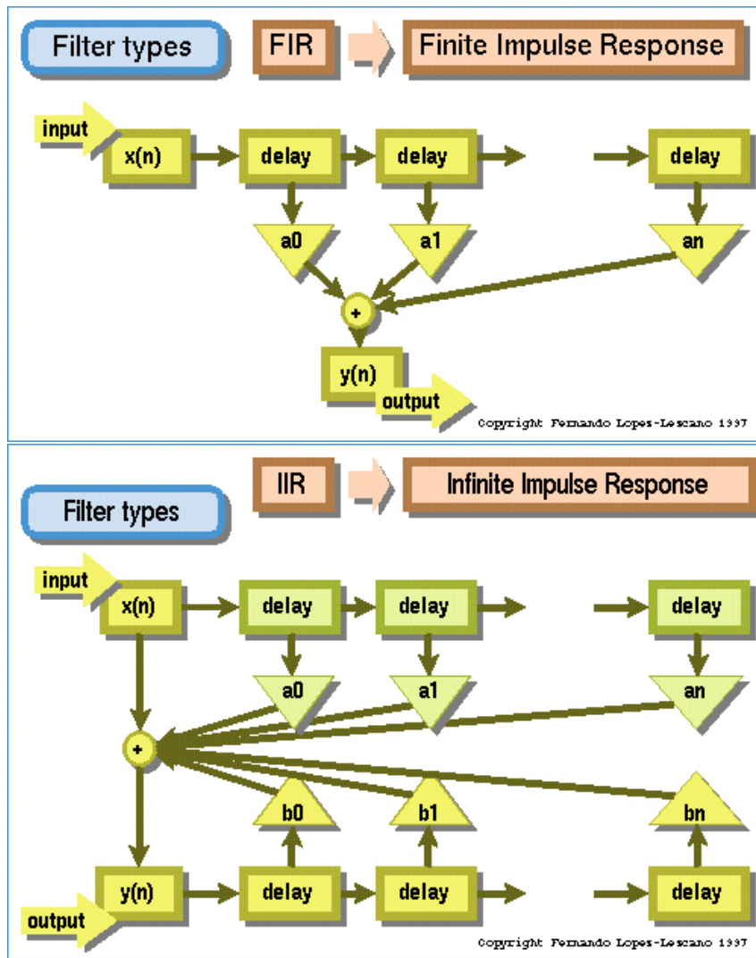
Figure 6: FIR and IIR filters. Filters are usually designed in the time domain, by delaying a signal and then averaging (in a wide variety of ways) the delayed signal and the nondelayed one. These are called finite impulse response ( FIR ) filters, because what comes out uses a finite number of samples, and a sample only has a finite effect.
