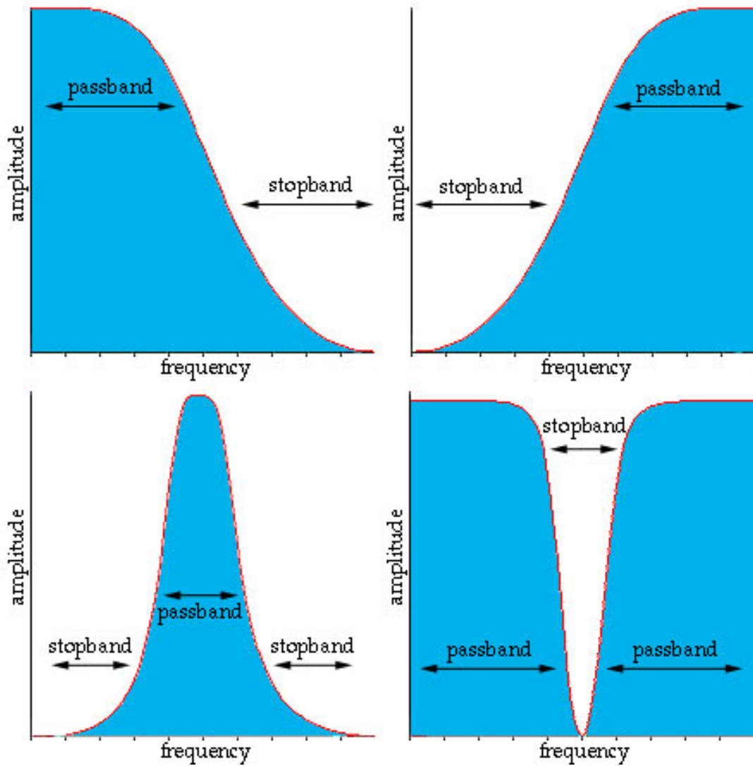
Figure 5: Four common filter types (clockwise from upper left): low-pass, high-pass, band-reject, band-pass.
