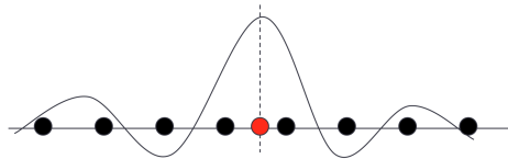
Figure 3: To resample a signal, we need to interpolate between existing samples in order to “reconstruct” the signal at a new time. A sequence of these new samples at a narrower or wider spacing creates a representation of the signal at a new sample rate. For each of these new samples (in this figure, the new sample will be at the dotted line), we form a weighted sum of existing samples. The weights are given by the so-called sinc function shown here (the thin wavy line). This weighted sum is essentially a low-pass filter that does in the digital domain what the reconstruction filter does in the analog domain when converting a digital signal to analog.
